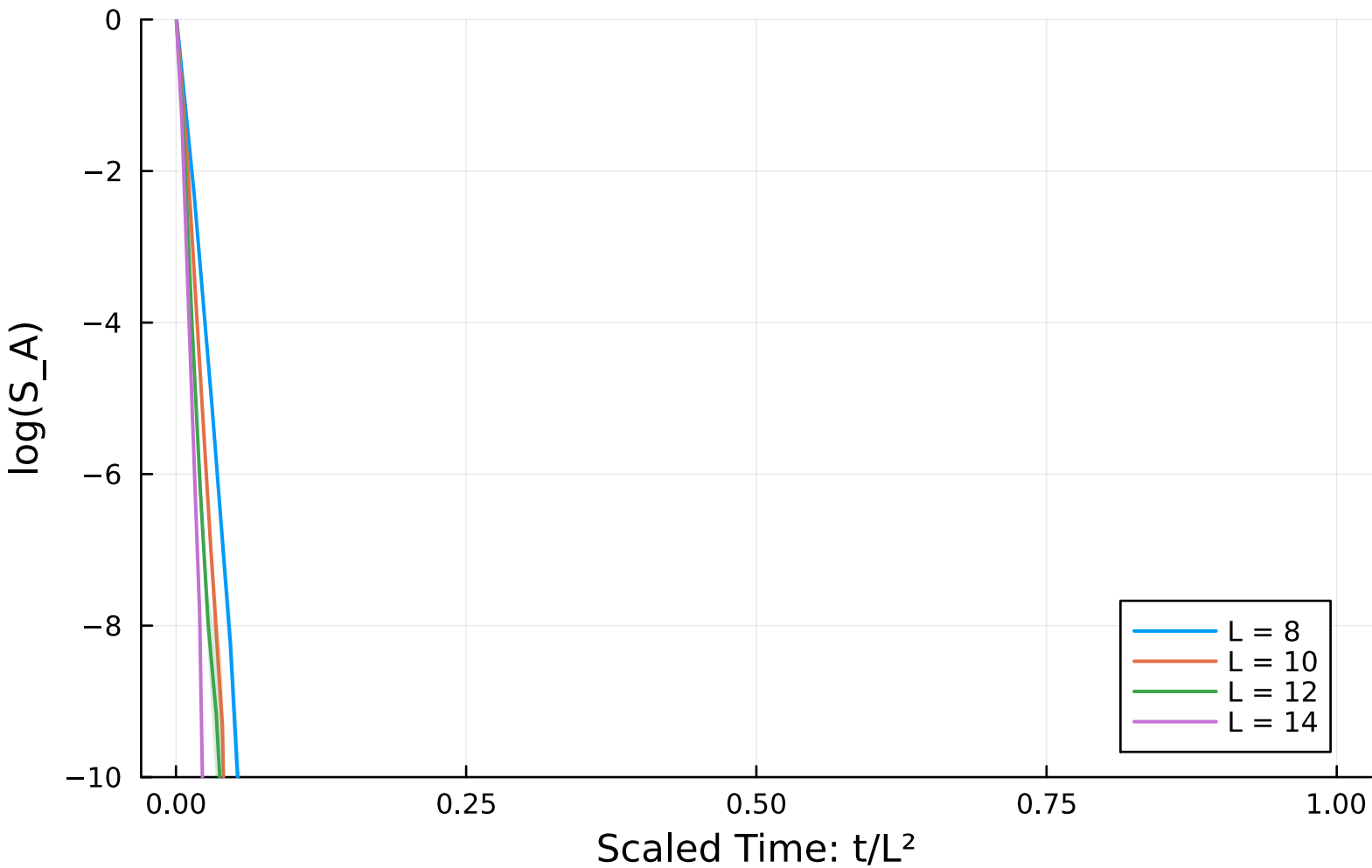
Scaled Log Entropy Evolution ( p = 0.916667 )
